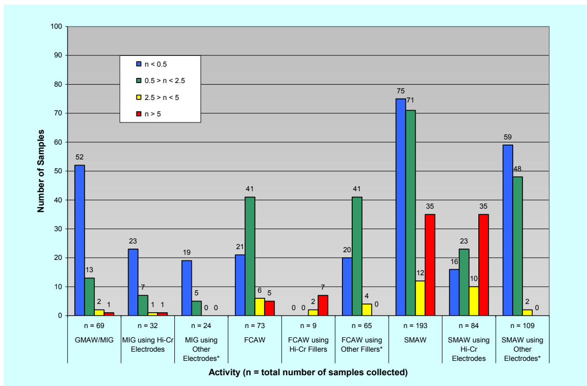
Figure 2. Comparison of CrVI Exposures (in \mu\text{g}/\text{m}^3 ) Based on Filler/Electrode Composition.
