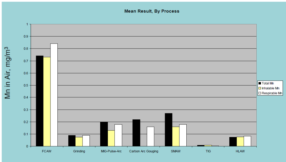
Figure 3. Comparison of Average Mn Fume, by Size Fraction, Measured During Shipyard Welding Activities
